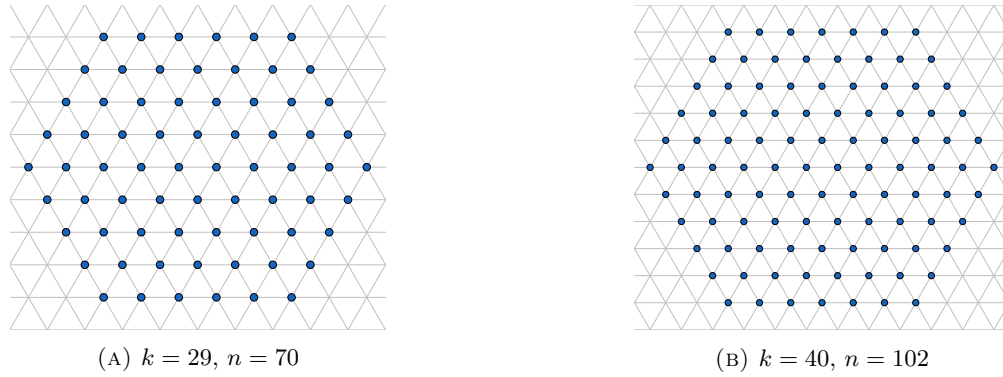
FIGURE 3. These two configurations show that g(k) > 2k + 1 for k \in \{30, 31, 32, 33, 45\} .
