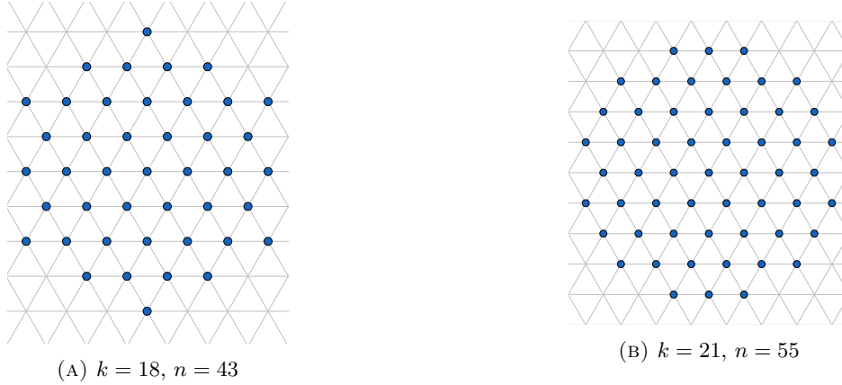
FIGURE 2. These two configurations show that g(k) > 2k + 1 for k \in \{18, 19, 20, 21, 22\} .
